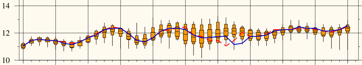
Precip. 3-hourly (mm)
