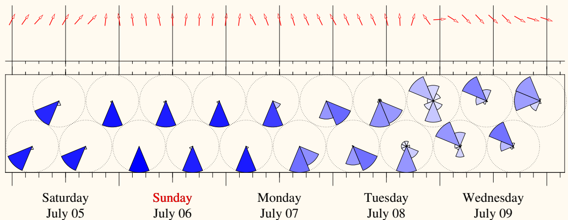
Distribution of 10m Wind Direction
