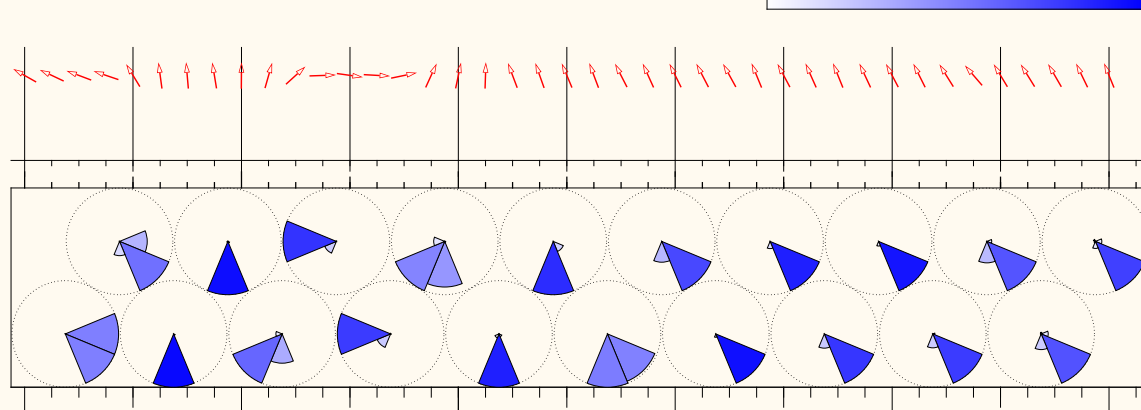
Distribution of 10m Wind Direction
