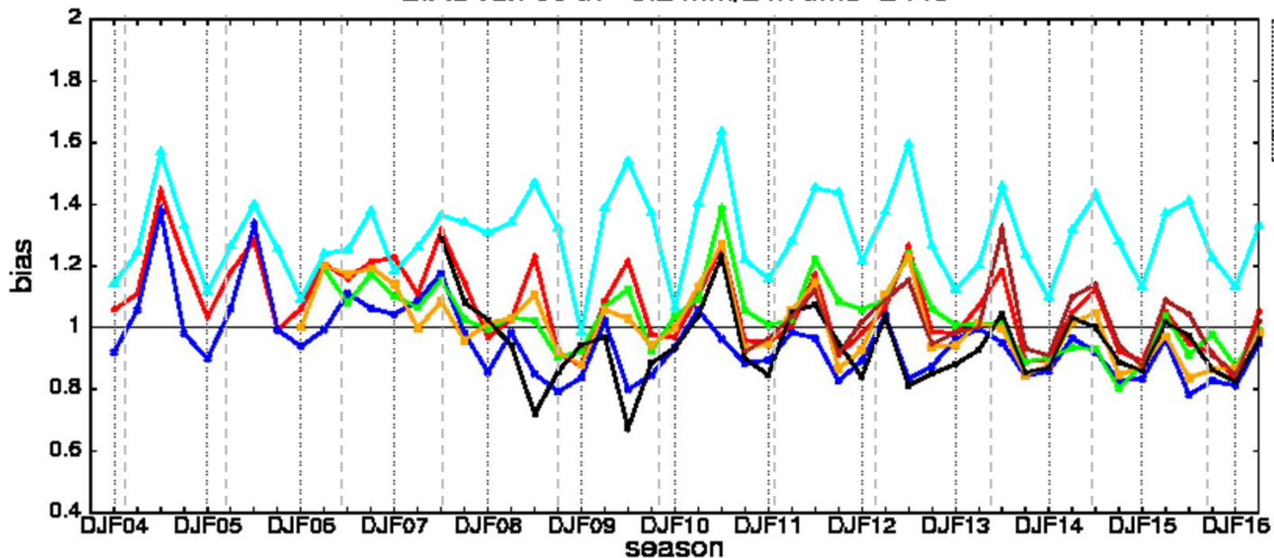
BIAS run 00 th= 0.2 mm/24h time=2448
